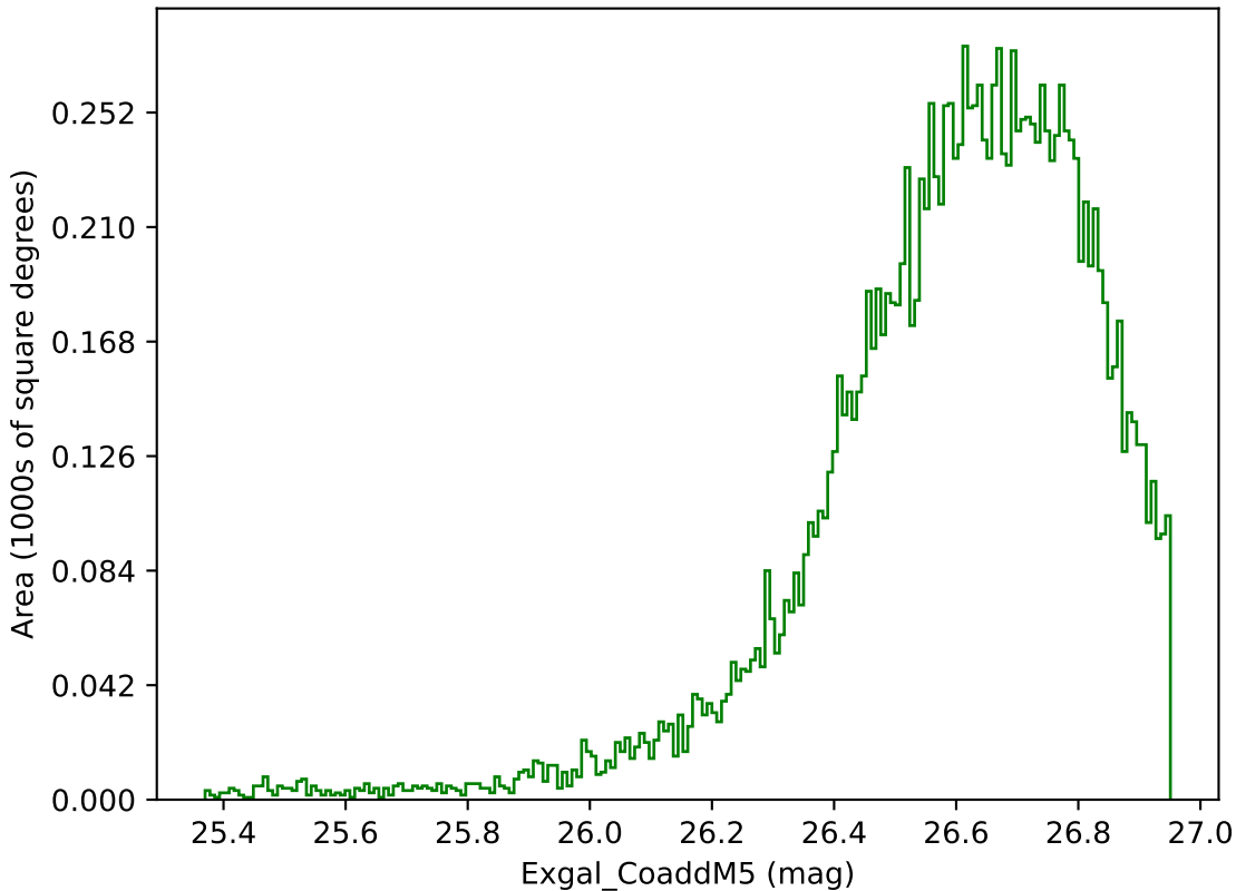
roman_v3.3_10yrs WFD g band: Exgal_CoaddM5
