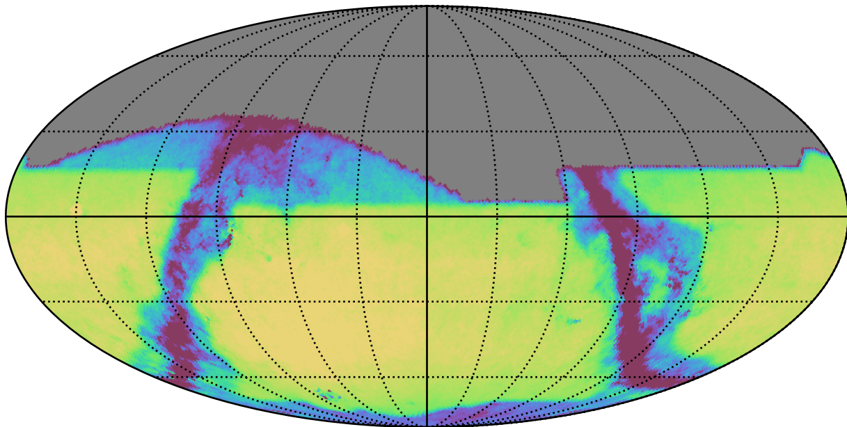
roman_v3.3_10yrs All sky z band: Exgal_CoaddM5
