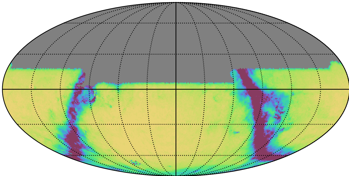
roman_v3.3_10yrs All sky u band: Exgal_CoaddM5
