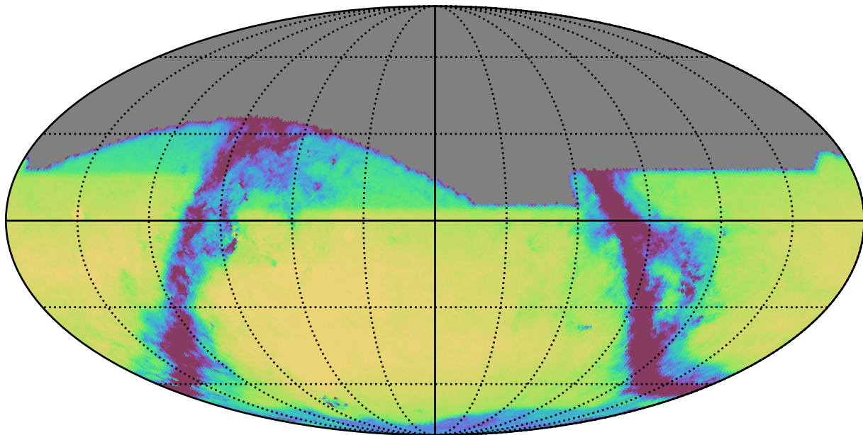
roman_v3.3_10yrs All sky r band: Exgal_CoaddM5
