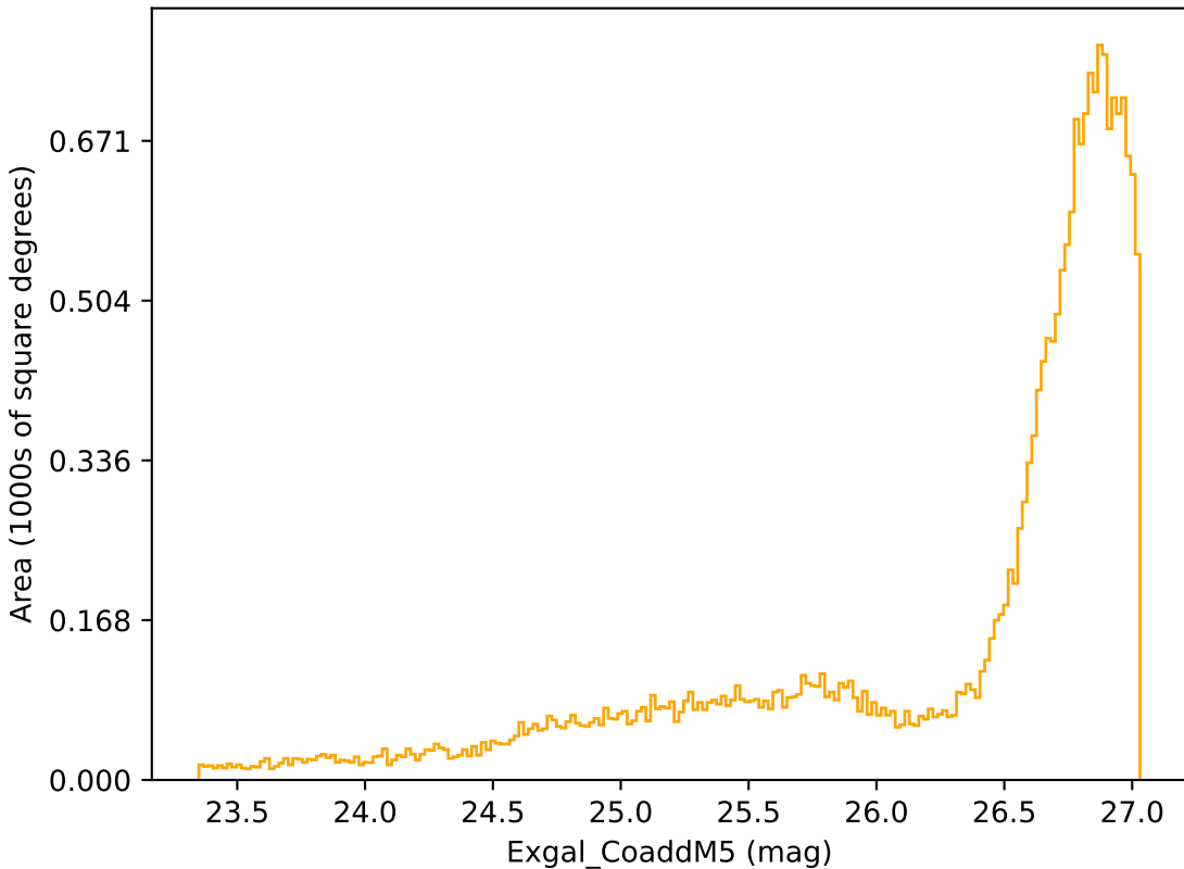
roman_v3.3_10yrs All sky r band: Exgal_CoaddM5
