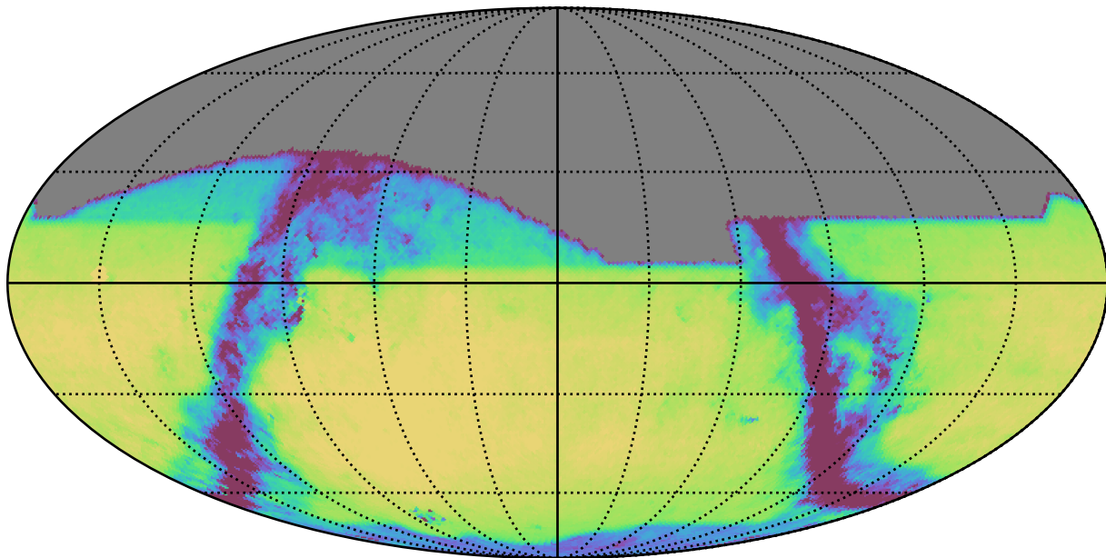
roman_v3.3_10yrs All sky i band: Exgal_CoaddM5
