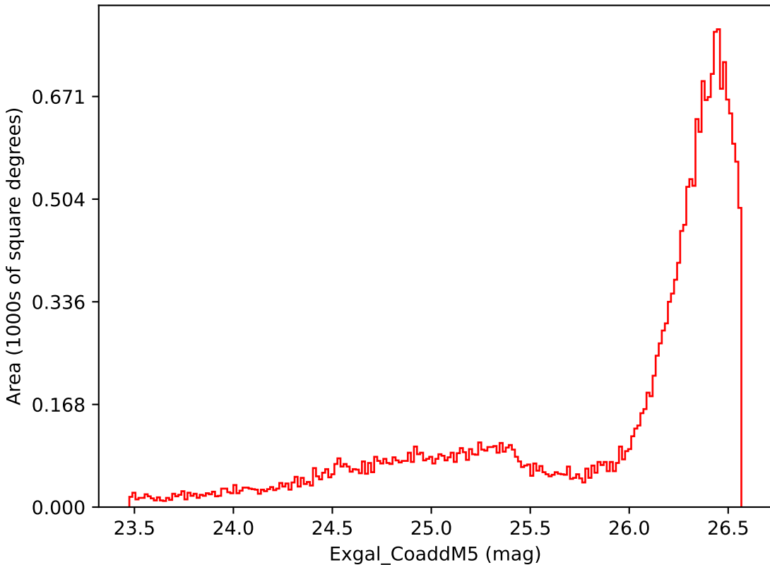
roman_v3.3_10yrs All sky i band: Exgal_CoaddM5
