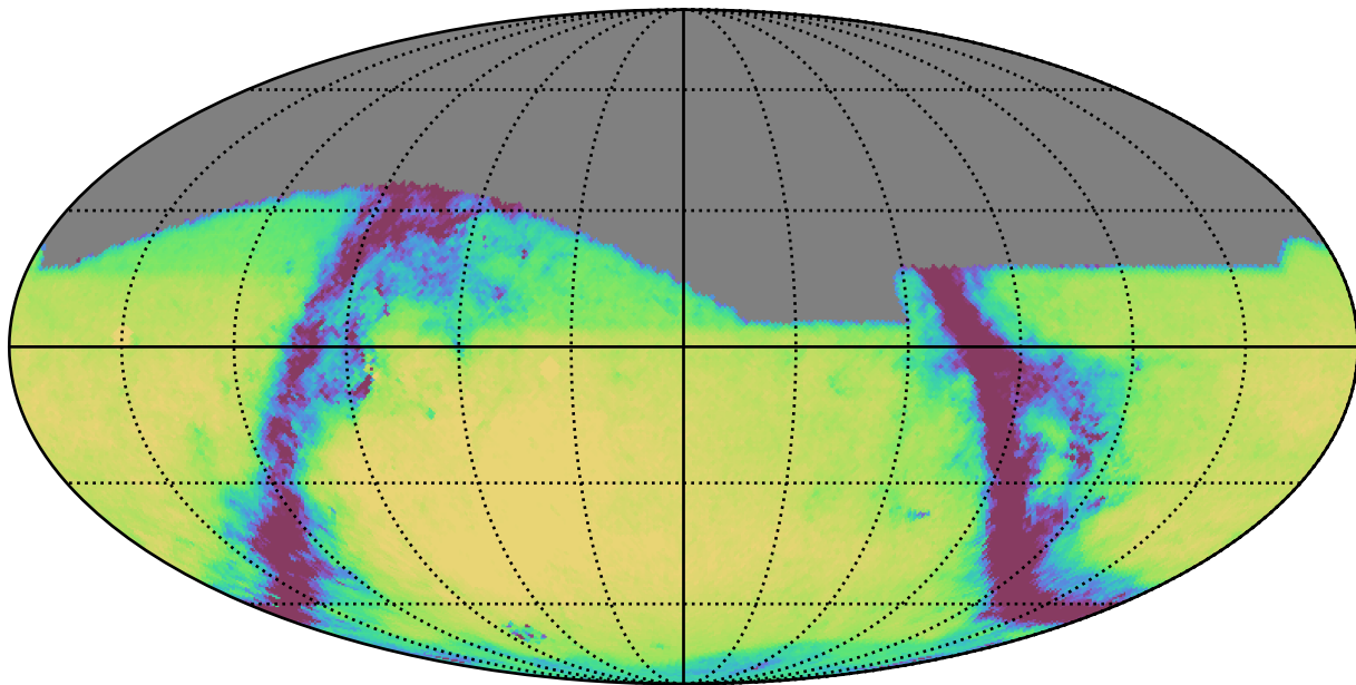
roman_v3.3_10yrs All sky g band: Exgal_CoaddM5
