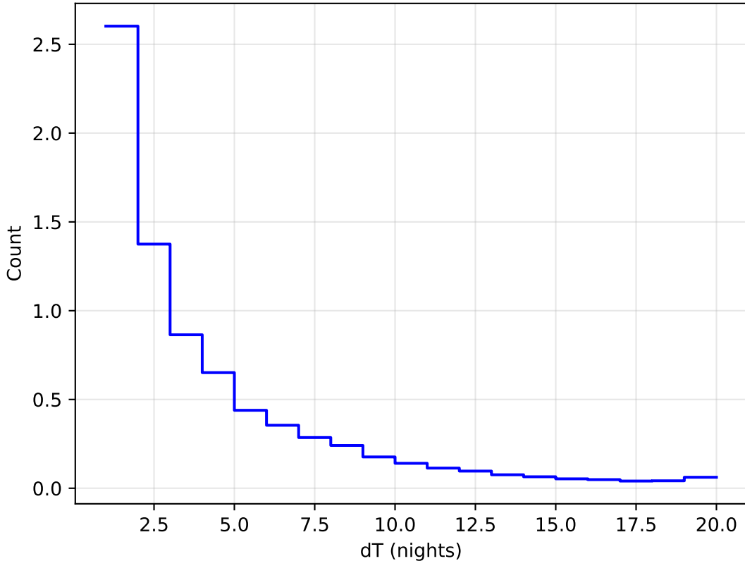
roman_v3.3_10yrs WFD all bands: DeltaNight Histogram
