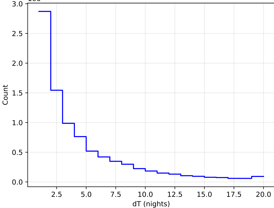
roman_v3.3_10yrs All sky all bands: DeltaNight Histogram 1e6
