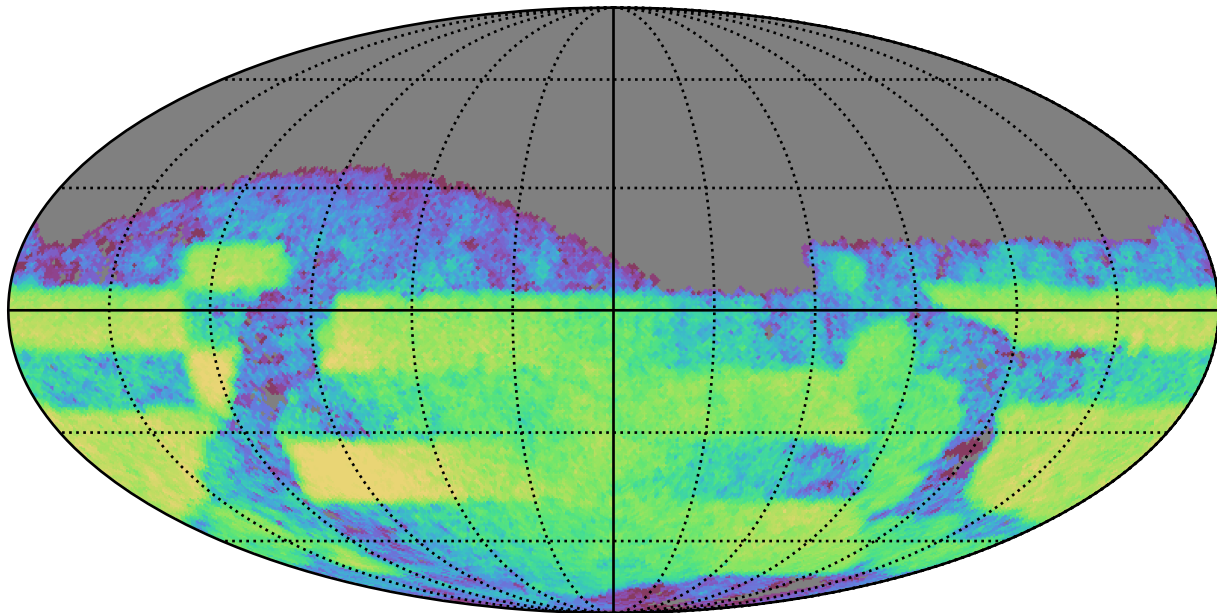
roman_v3.3_10yrs Yr 3-4 z band: CoaddM5
