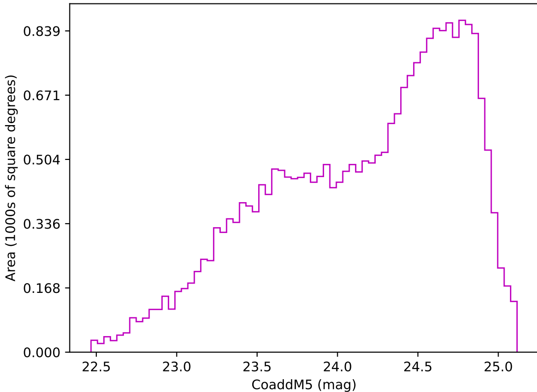
roman_v3.3_10yrs Yr 3-4 z band: CoaddM5
