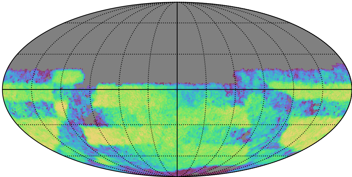
roman_v3.3_10yrs Yr 3-4 y band: CoaddM5
