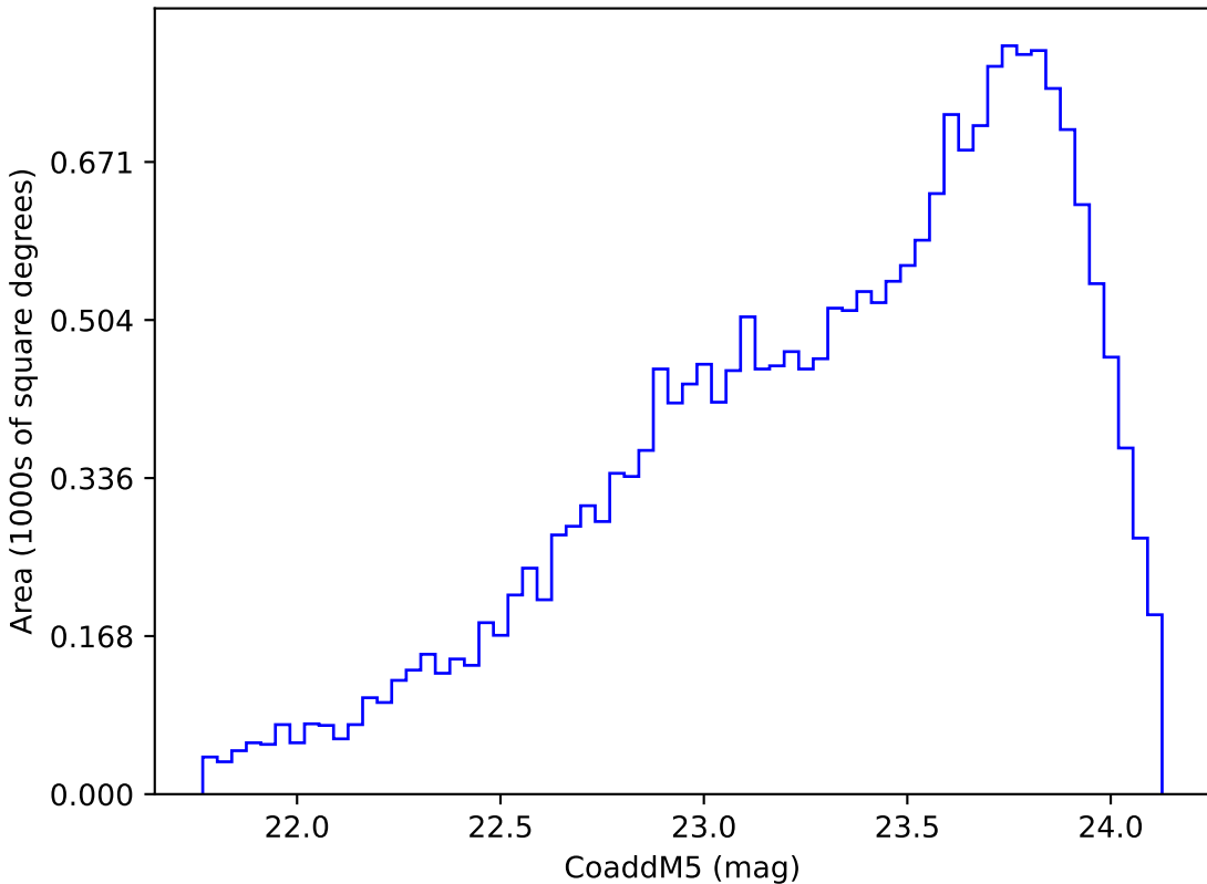
roman_v3.3_10yrs Yr 3-4 y band: CoaddM5
