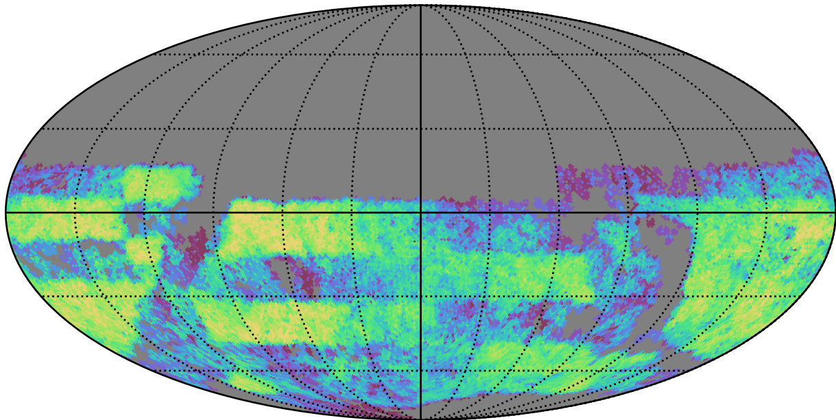
roman_v3.3_10yrs Yr 3-4 u band: CoaddM5
