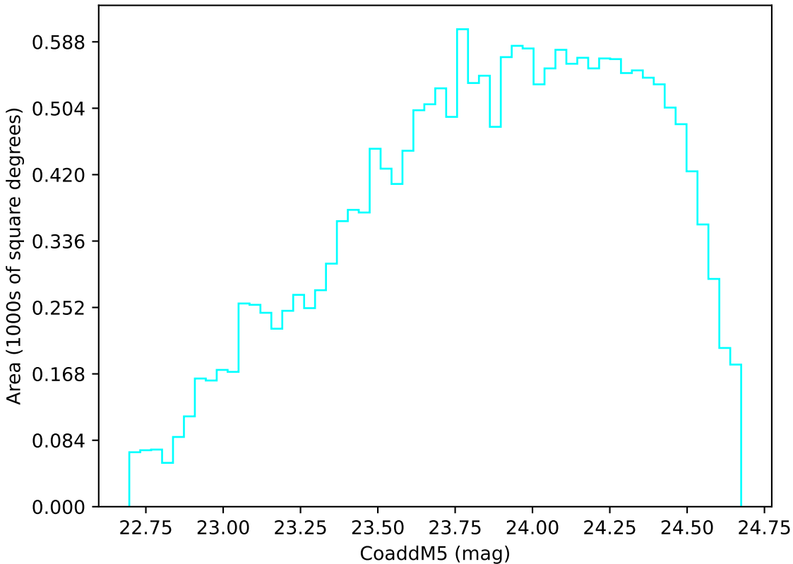
roman_v3.3_10yrs Yr 3-4 u band: CoaddM5
