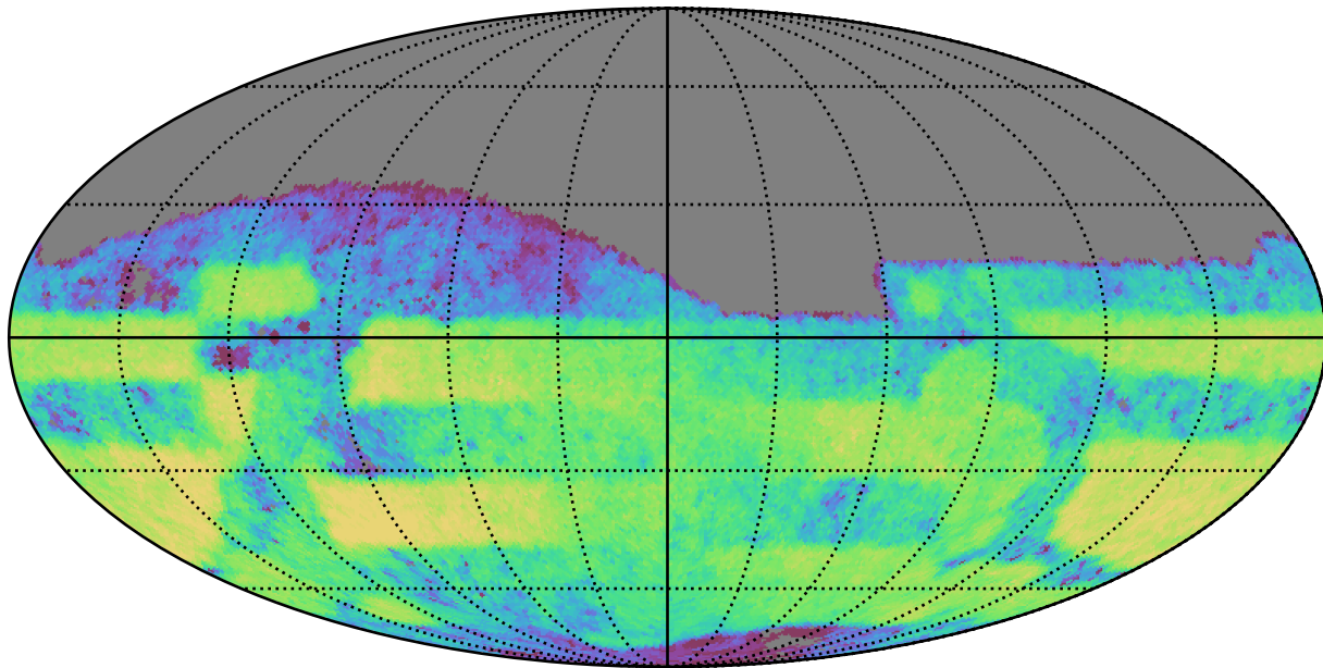
roman_v3.3_10yrs Yr 3-4 r band: CoaddM5
