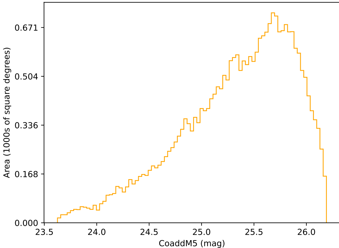
roman_v3.3_10yrs Yr 3-4 r band: CoaddM5
