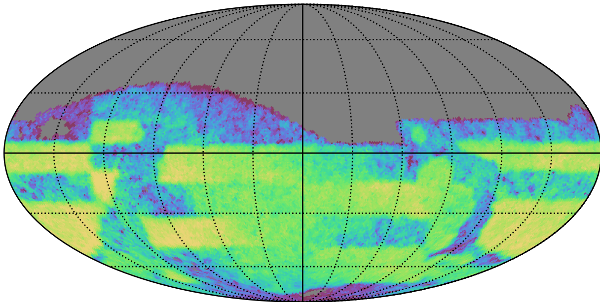
roman_v3.3_10yrs Yr 3-4 i band: CoaddM5
