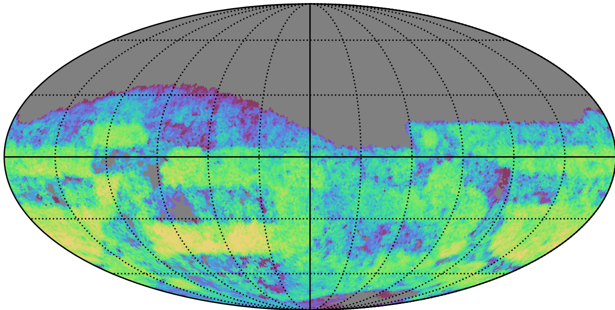
roman_v3.3_10yrs Yr 3-4 g band: CoaddM5
