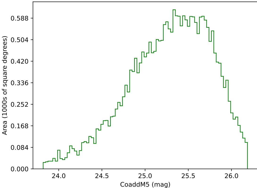
roman_v3.3_10yrs Yr 3-4 g band: CoaddM5
