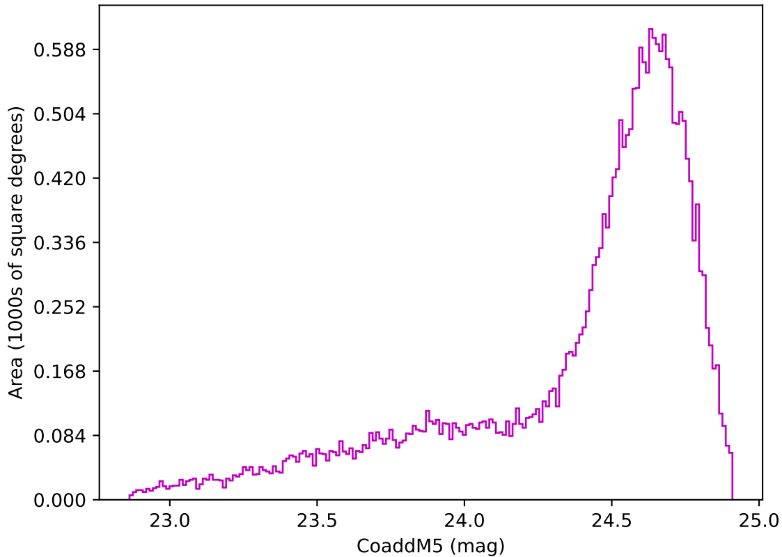
roman_v3.3_10yrs Yr 1 z band: CoaddM5
