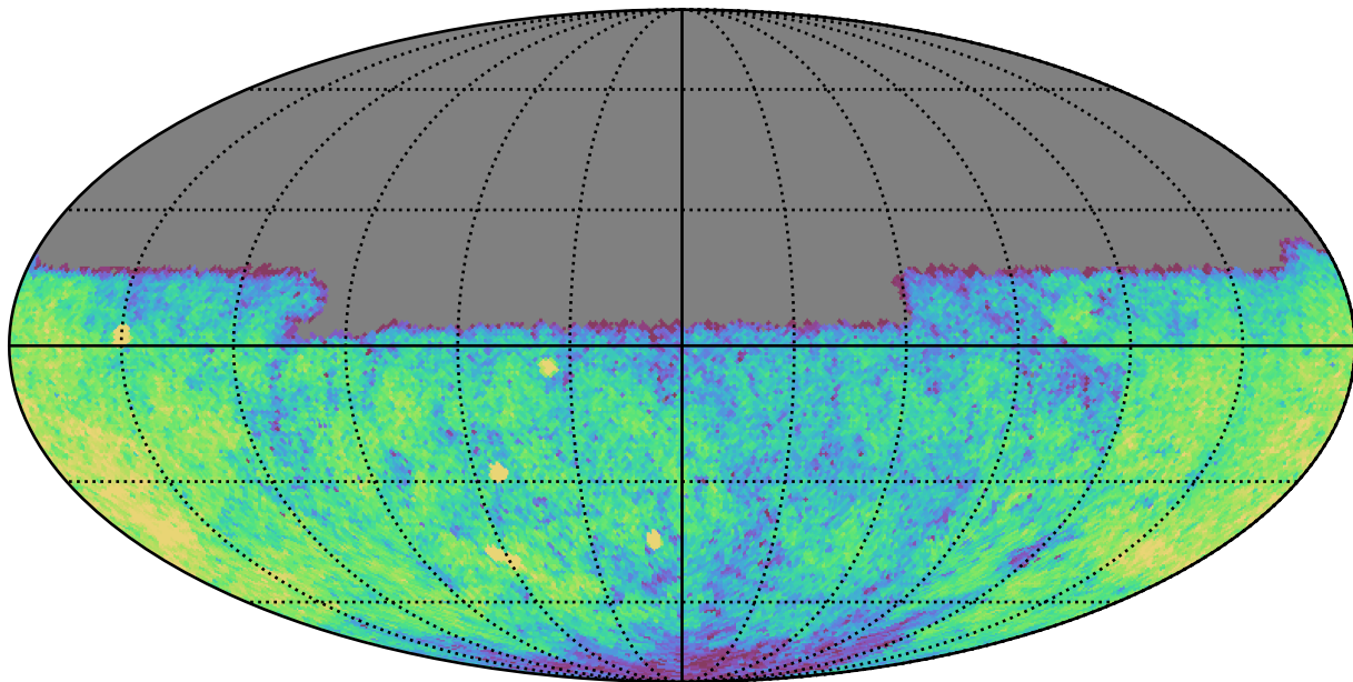
roman_v3.3_10yrs Yr 1 u band: CoaddM5
