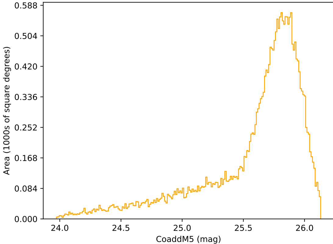
roman_v3.3_10yrs Yr 1 r band: CoaddM5
