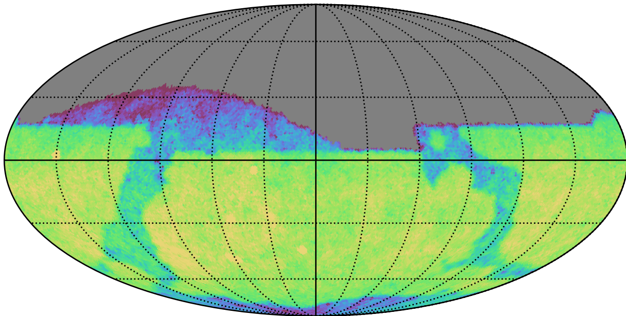
roman_v3.3_10yrs Yr 1 i band: CoaddM5
