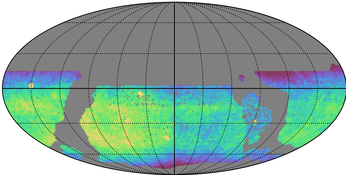
roman_v3.3_10yrs WFD z band: CoaddM5
