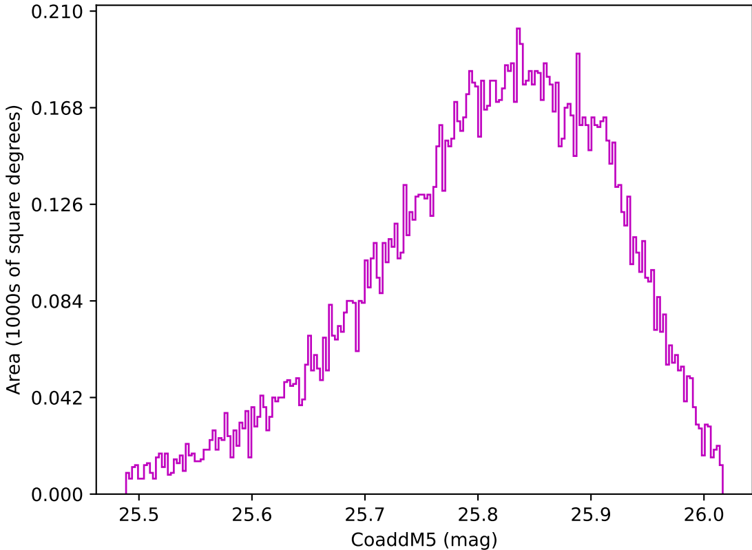
roman_v3.3_10yrs WFD z band: CoaddM5
