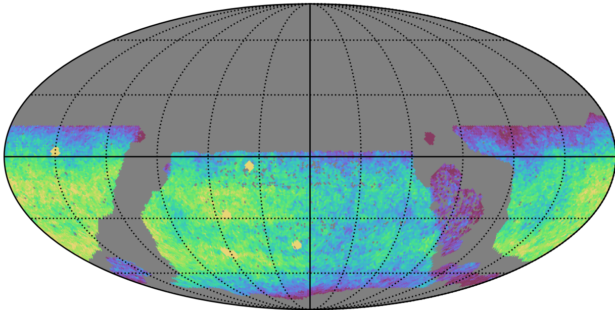
roman_v3.3_10yrs WFD u band: CoaddM5
