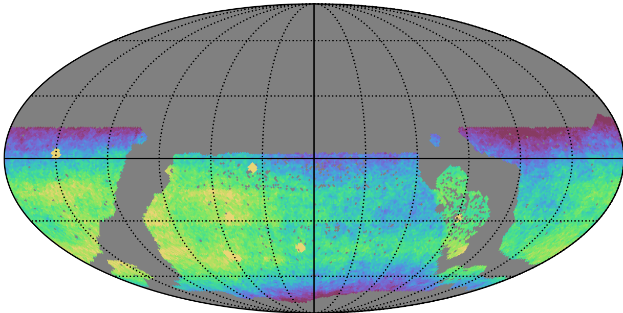
roman_v3.3_10yrs WFD r band: CoaddM5
