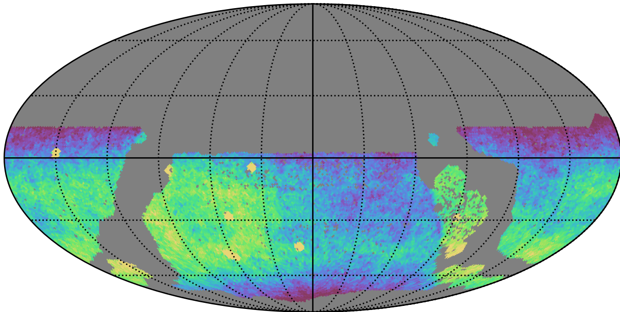
roman_v3.3_10yrs WFD g band: CoaddM5
