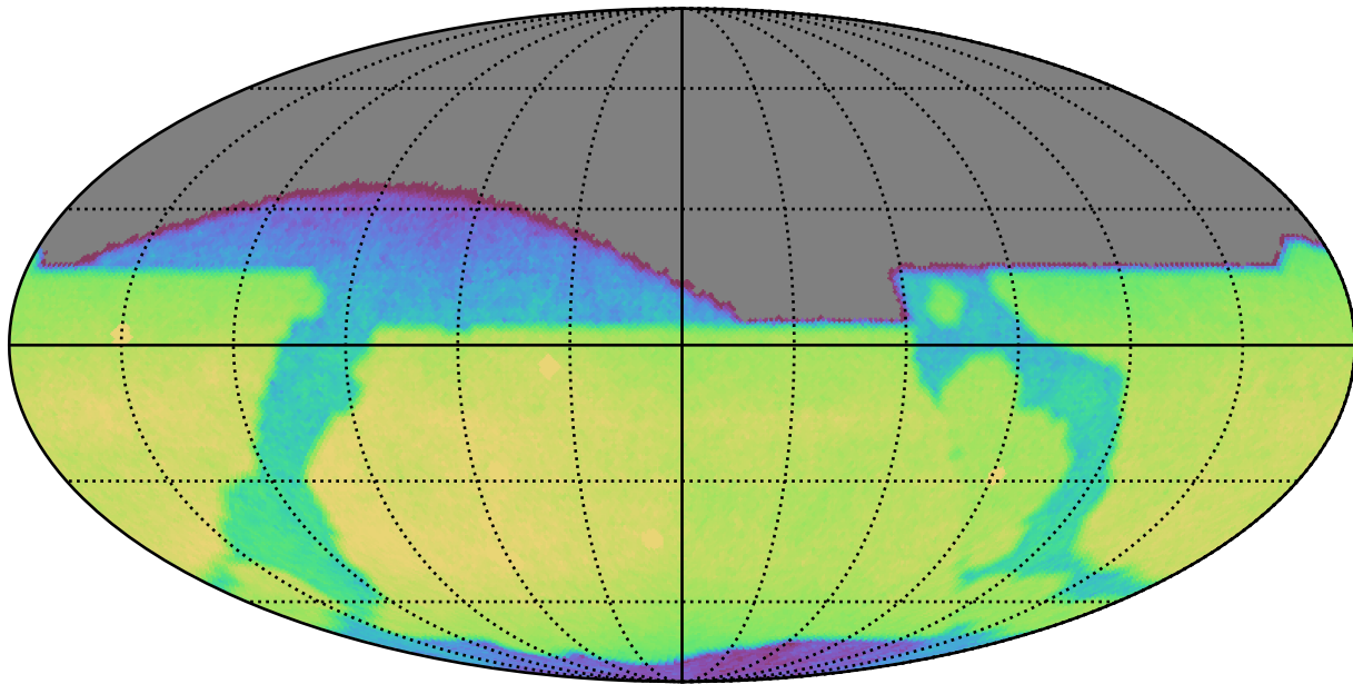
roman_v3.3_10yrs All sky z band: CoaddM5
