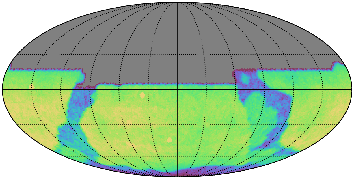
roman_v3.3_10yrs All sky u band: CoaddM5
