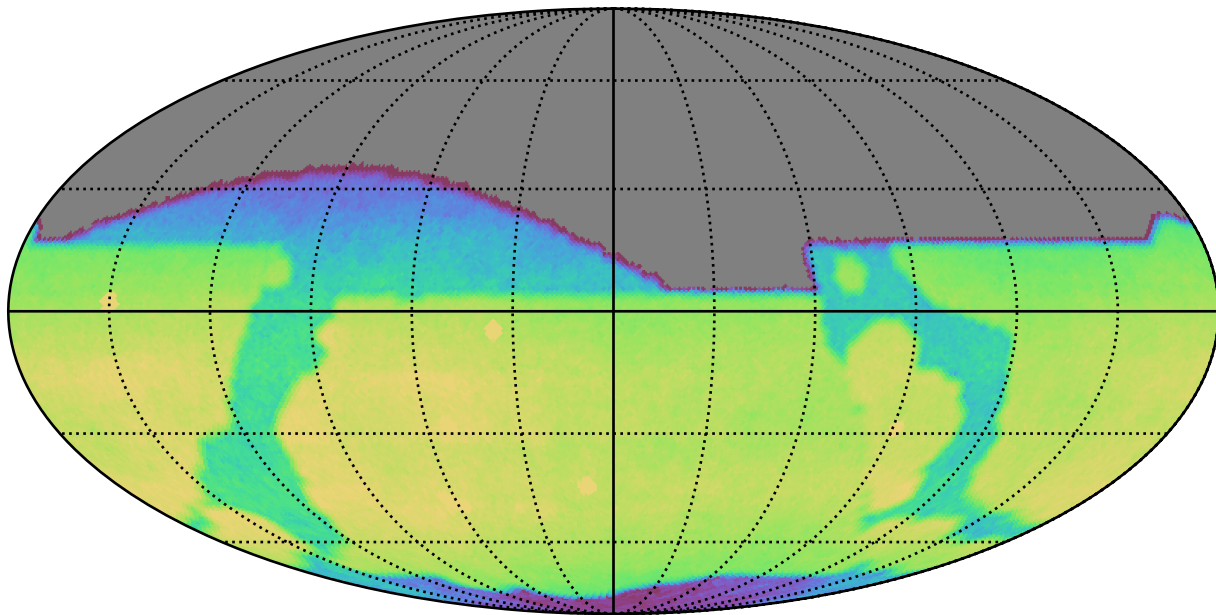
roman_v3.3_10yrs All sky r band: CoaddM5
