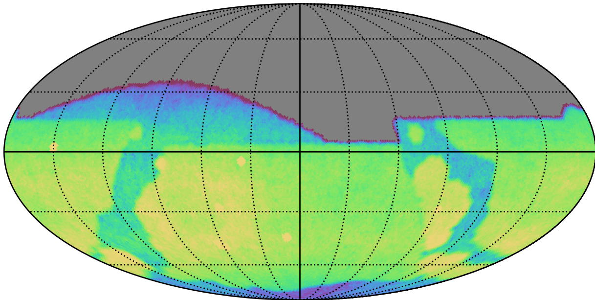
roman_v3.3_10yrs All sky g band: CoaddM5
