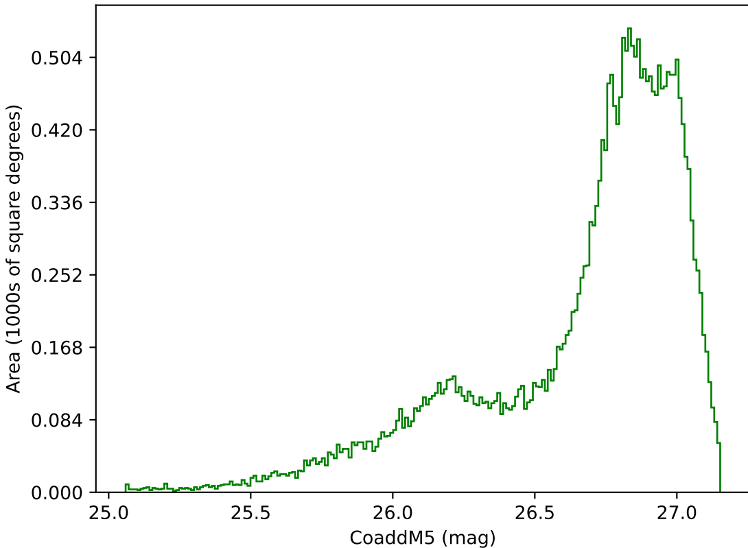
roman_v3.3_10yrs All sky g band: CoaddM5
