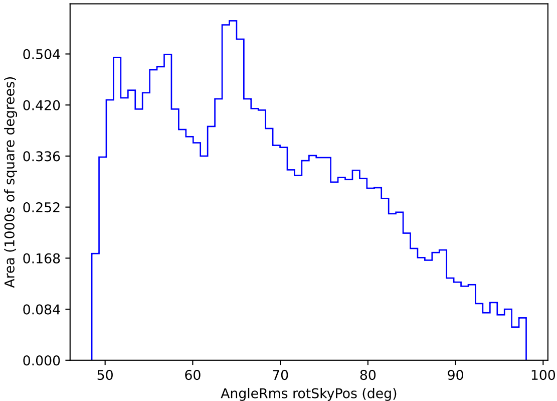
roman_v3.3_10yrs WFD all bands: AngleRms rotSkyPos
