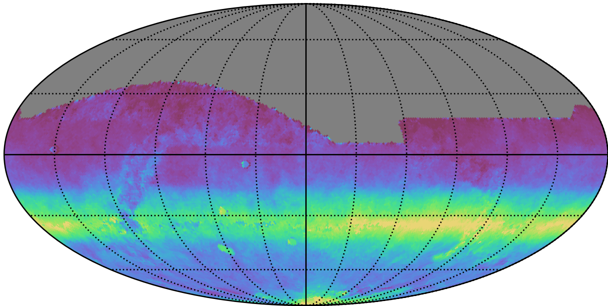
roman_v3.3_10yrs All sky all bands: AngleRms rotSkyPos
