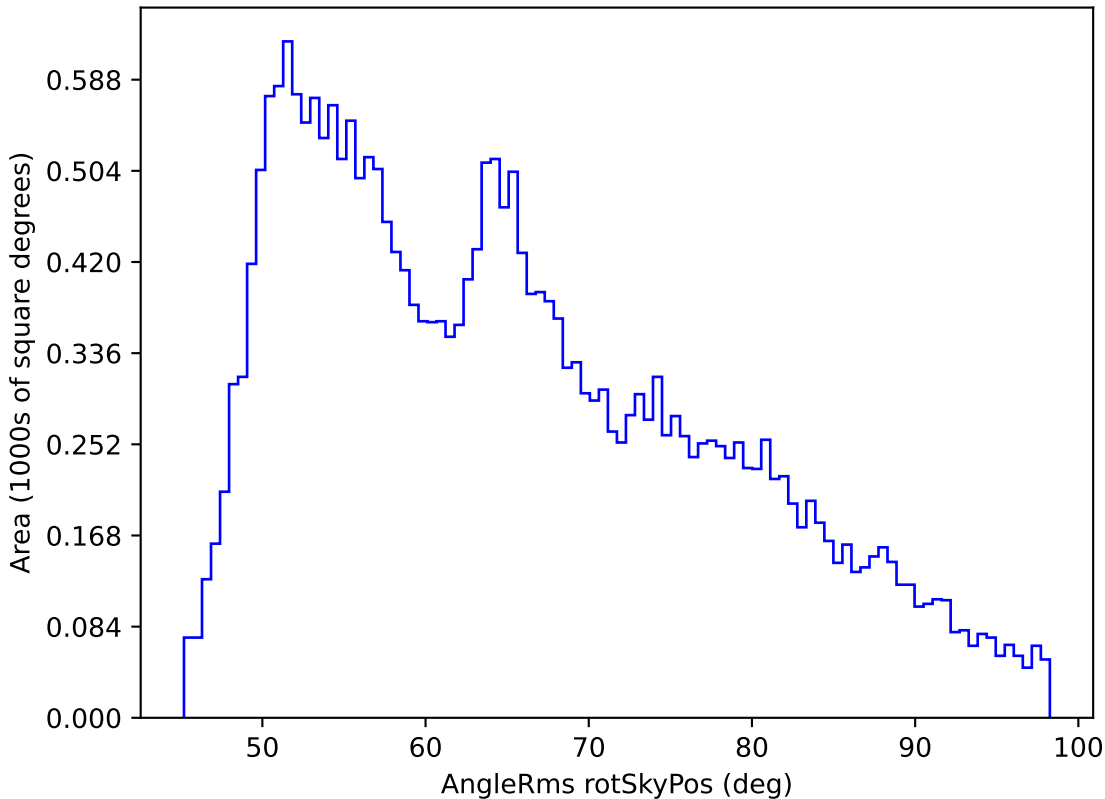
roman_v3.3_10yrs All sky all bands: AngleRms rotSkyPos
