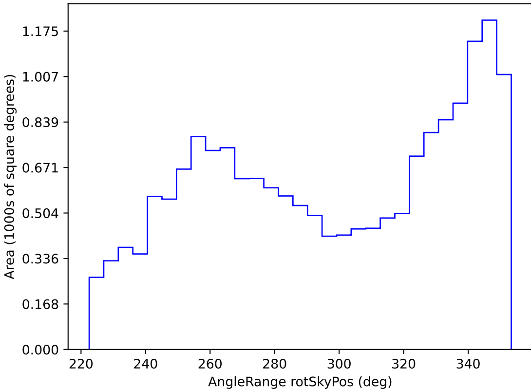
roman_v3.3_10yrs WFD all bands: AngleRange rotSkyPos
