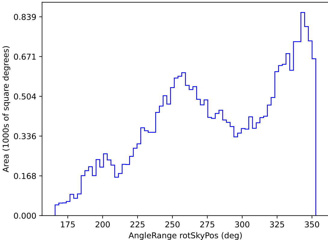
roman_v3.3_10yrs All sky all bands: AngleRange rotSkyPos
