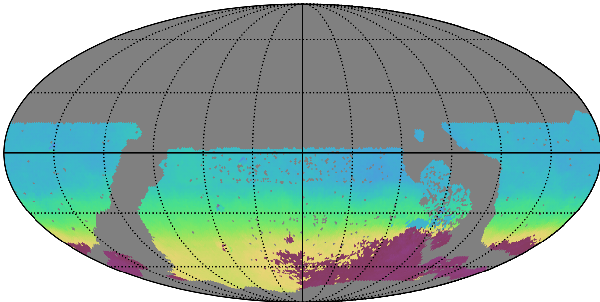
roman_v3.3_10yrs WFD all bands: AngleMean rotSkyPos
