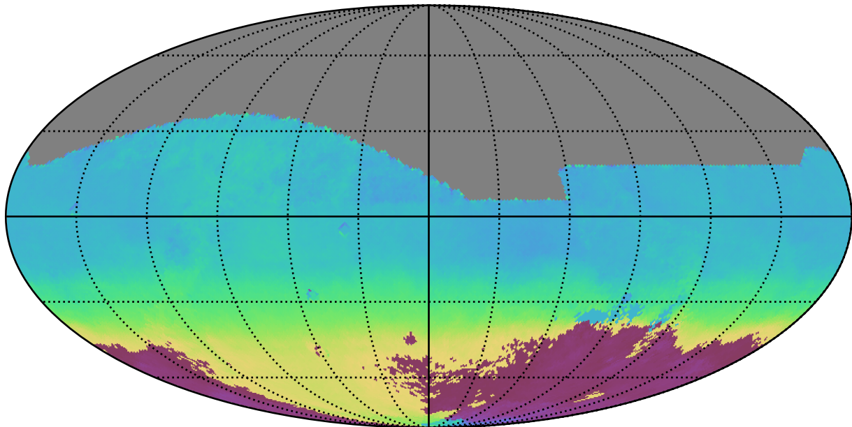
roman_v3.3_10yrs All sky all bands: AngleMean rotSkyPos
