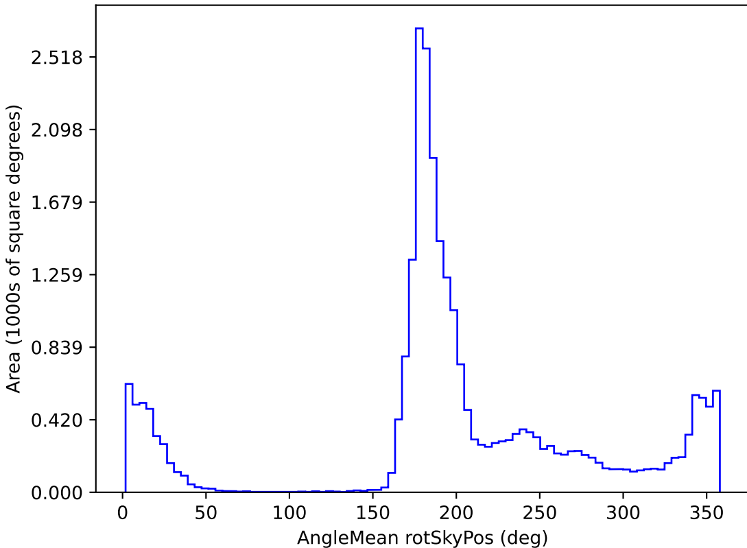
roman_v3.3_10yrs All sky all bands: AngleMean rotSkyPos
