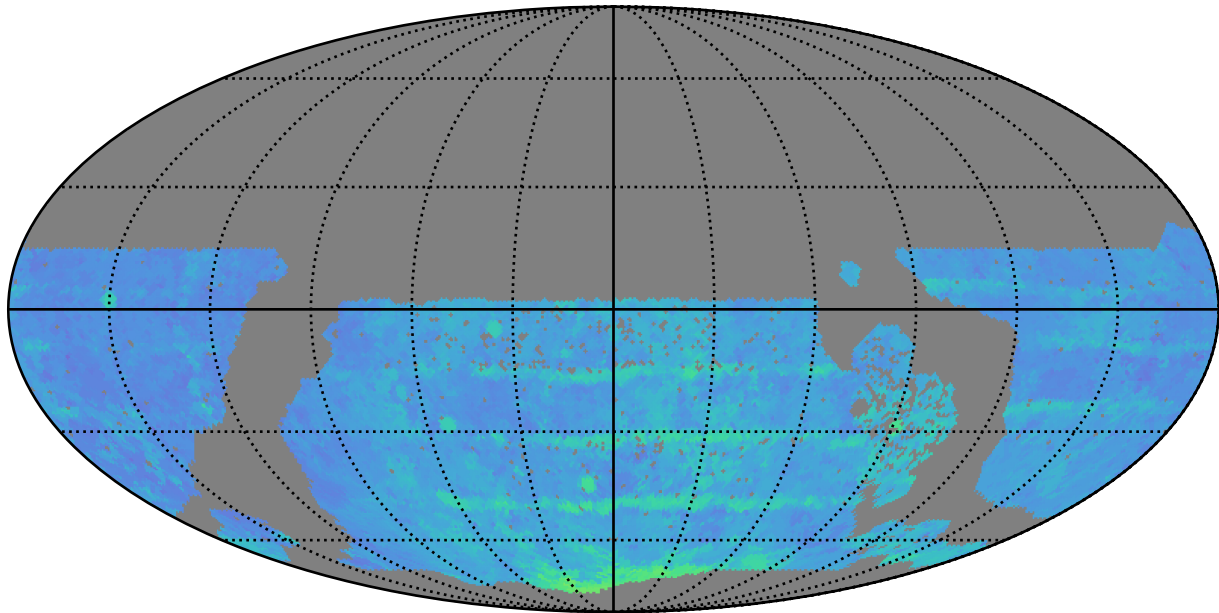
roman_v3.3_10yrs WFD z band: 80thPercentile Season Length
