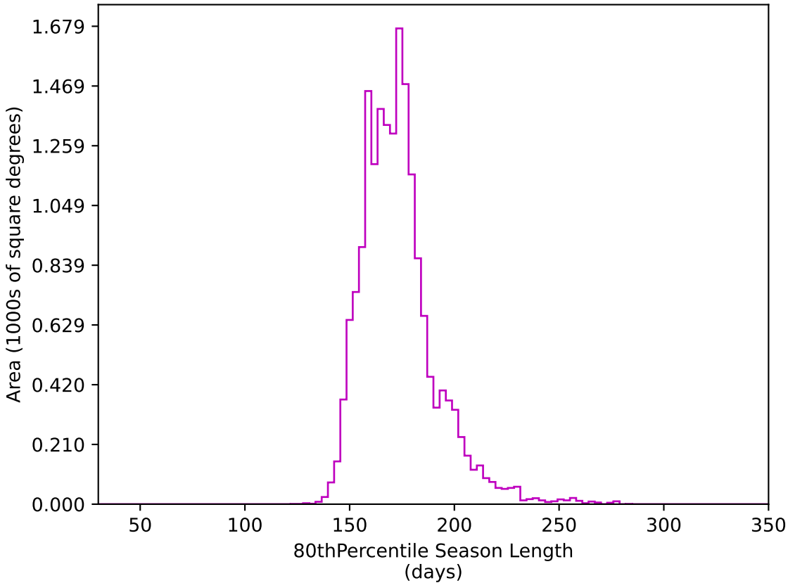
roman_v3.3_10yrs WFD z band: 80thPercentile Season Length
