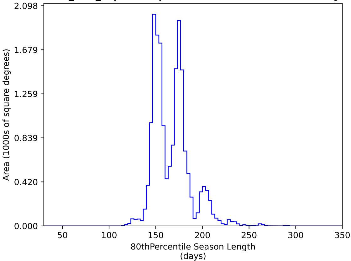
roman_v3.3_10yrs WFD y band: 80thPercentile Season Length
