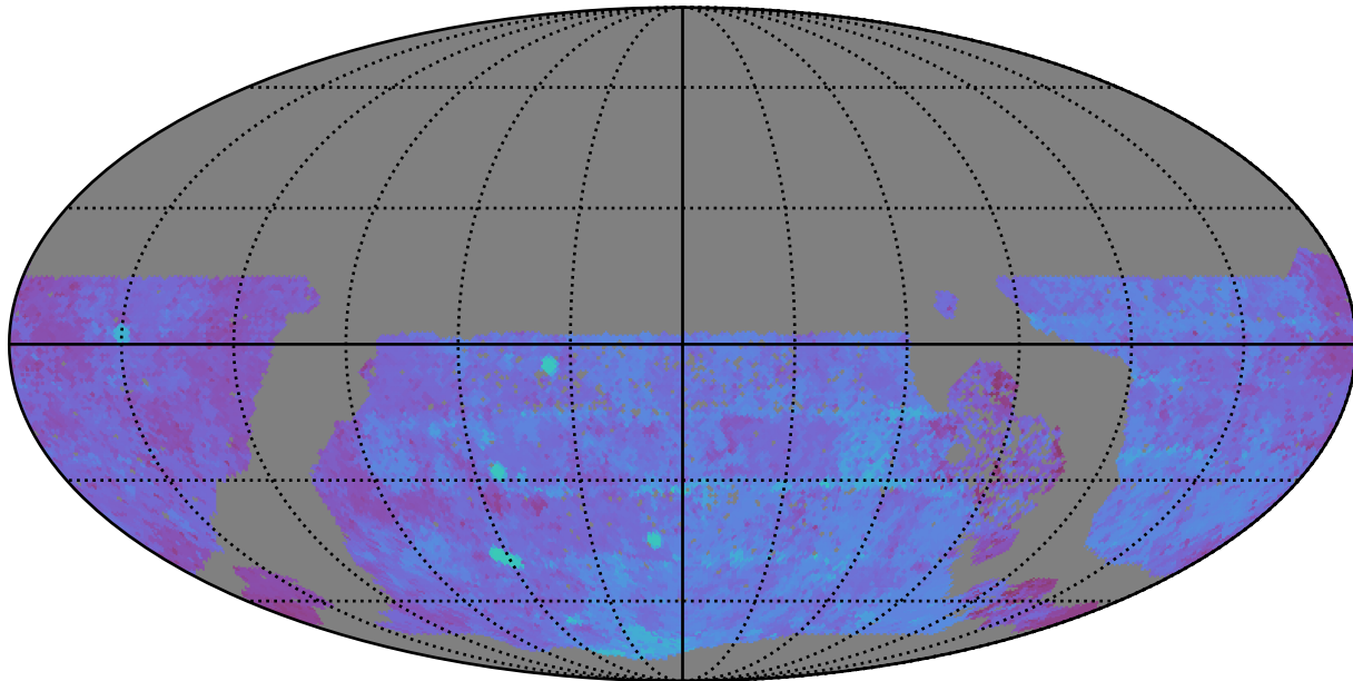
roman_v3.3_10yrs WFD u band: 80thPercentile Season Length
