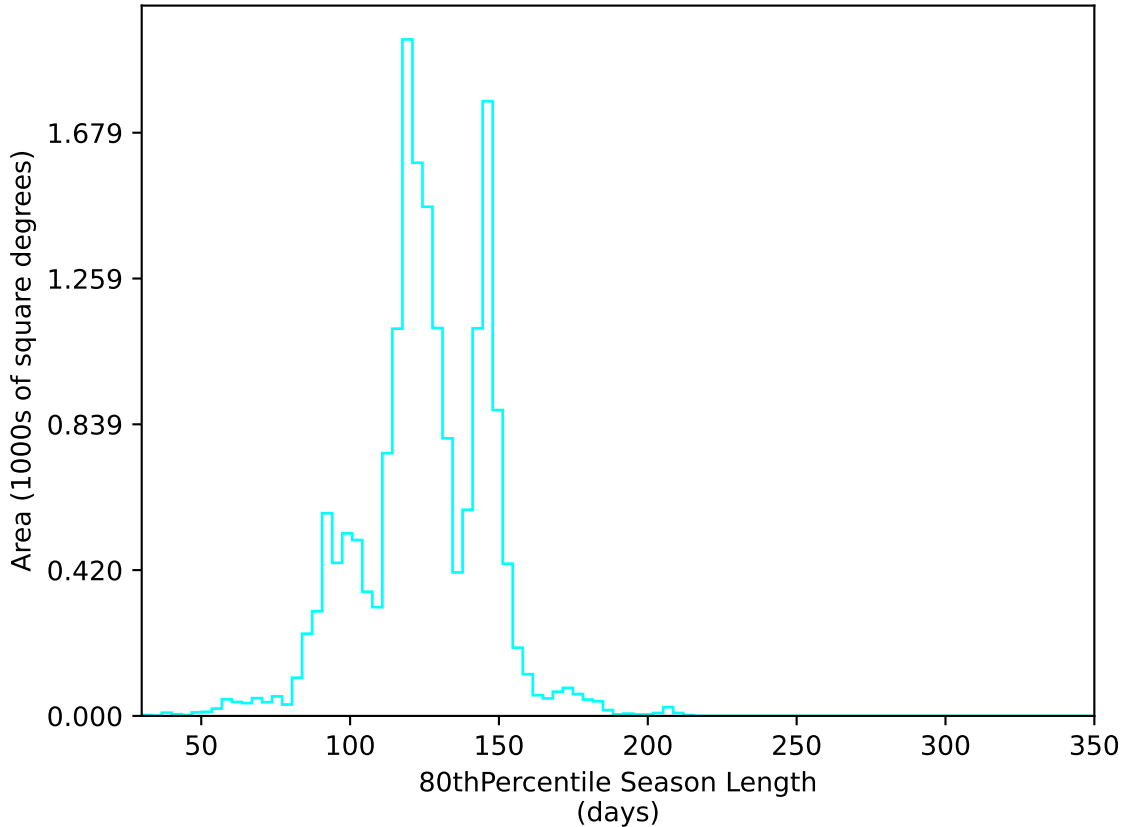
roman_v3.3_10yrs WFD u band: 80thPercentile Season Length
