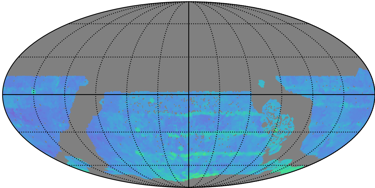
roman_v3.3_10yrs WFD r band: 80thPercentile Season Length
