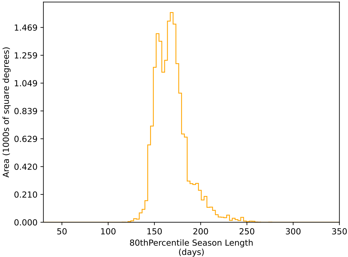
roman_v3.3_10yrs WFD r band: 80thPercentile Season Length
